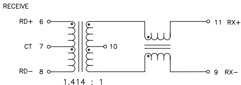
SCHEMATIC
