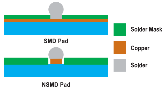
Figure 2. Comparison between solder mask defined pad and non-solder mask defined pad.
