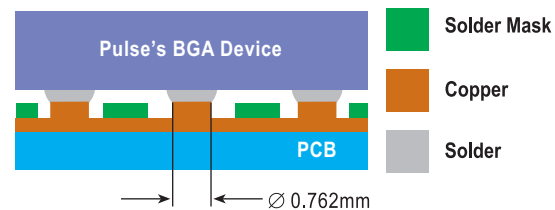
Figure 3. Recommend Land Pad for BGA device
